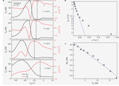
Figure 11: Taken from Fig. 4 in [4]. (a) Measurements of Hall resistivity R_{xy} and longitudinal resistivity R_{xx} , performed on the 80 nm thick sample, as a function of back gate voltage V_{bg} for several temperatures T at a magnetic field strength of B = 31 T. (b) Fit of the longitudinal conductivity \sigma_{xx} as a function of inverse temperature 1/T for \nu = 1 (blue dashed line is a fit for higher T ). (c) \Delta R_{xy}(T) = R_{xy}(T) - R_{xy}(T = 4.5 \text{ K}) versus R_{xx} for \nu = 1 (blue dashed line is a linear fit)
